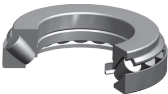
Bearing No. 294/800EM
