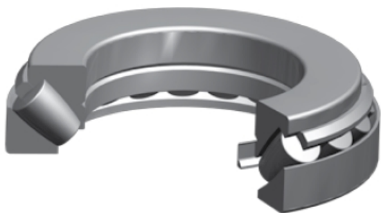
Bearing No. 294/670EM
