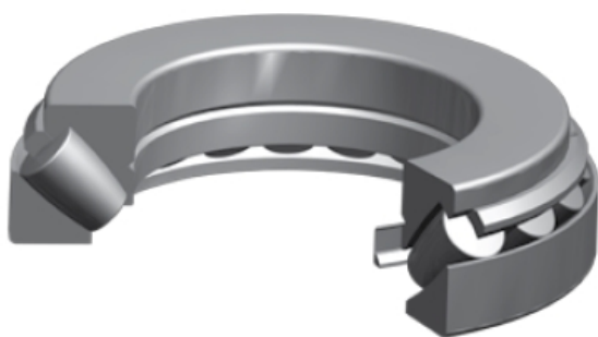
Bearing No. 29392EM
