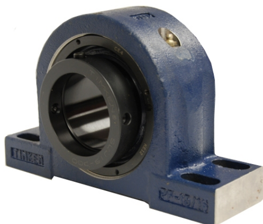
Bearing No. QMPX22J408S
