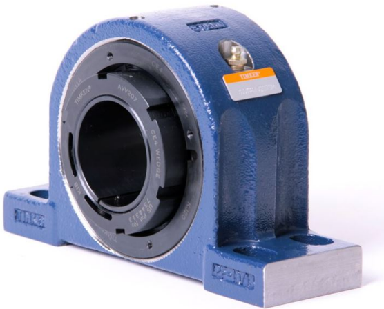
Bearing No. QVVPH22V311S
