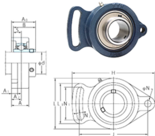
Bearing No. UCFA206-18
