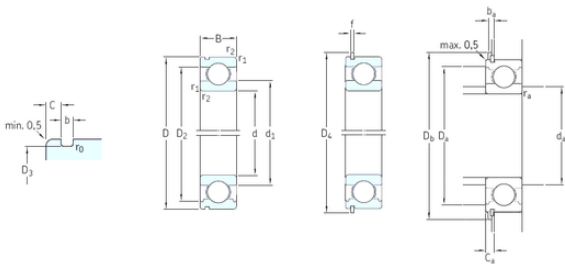
Bearing No. 6013N
