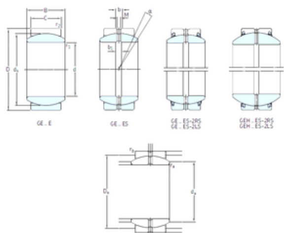
Bearing No. GE140ES
