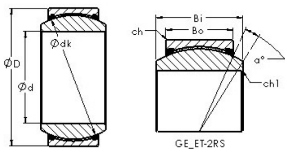
Bearing No. GEG30ET-2RS
