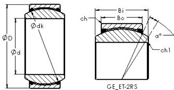
Bearing No. GEG60ET-2RS
