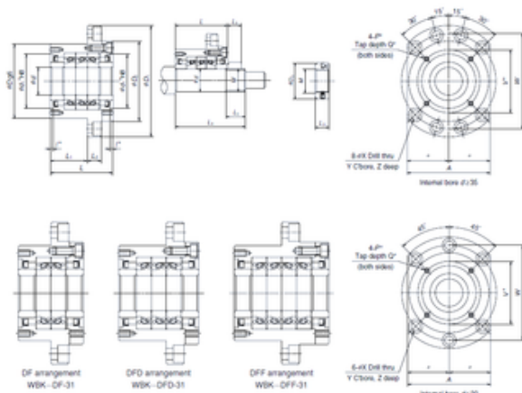
Bearing No. WBK40DFF-31
