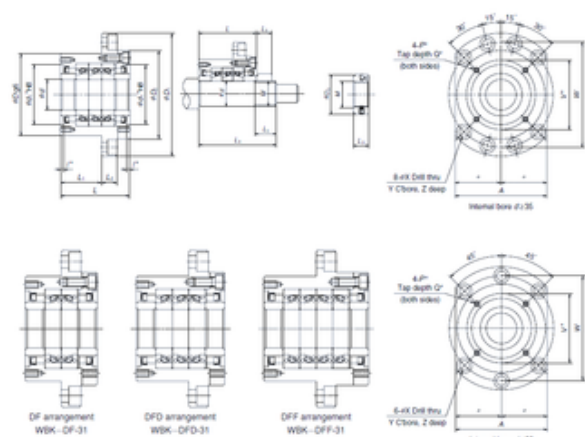
Bearing No. WBK35DFD-31
