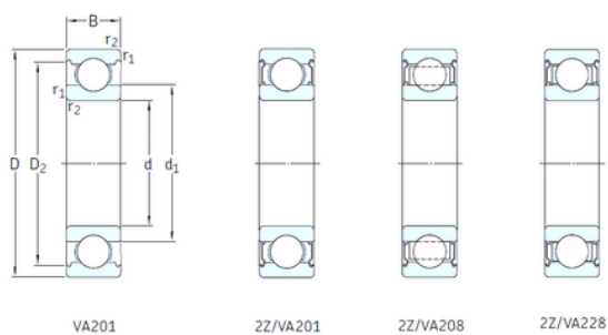
Bearing No. 6011-2Z/VA201
