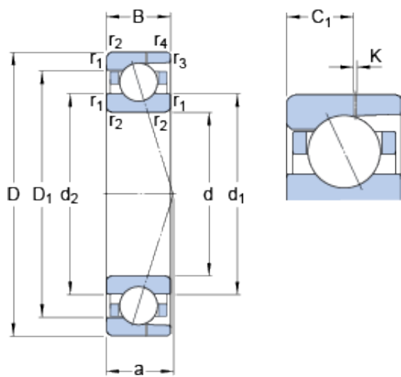
Bearing No. 7000 ACD/HCP4AH
