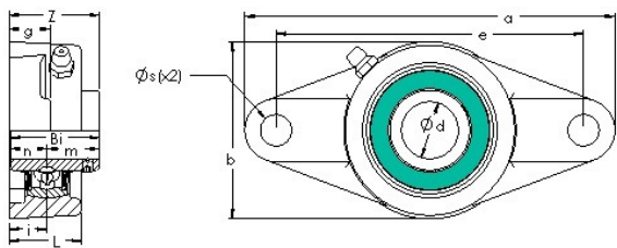
Bearing No. UCFL 207-20G5PL
