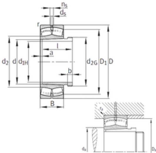
Bearing No. 23238-B-K-MB+AH3238G
