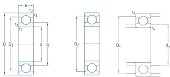
Bearing No. 6008
