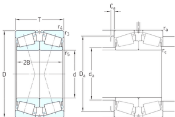
Bearing No. 30224J2/DF
