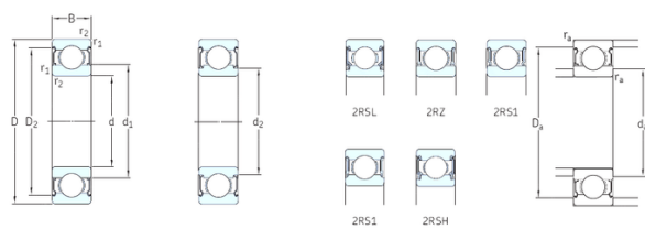
Bearing No. 6007-RS1
