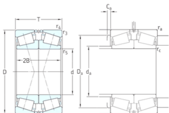
Bearing No. 30218J2/DF
