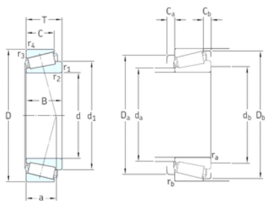
Bearing No. 30218J2
