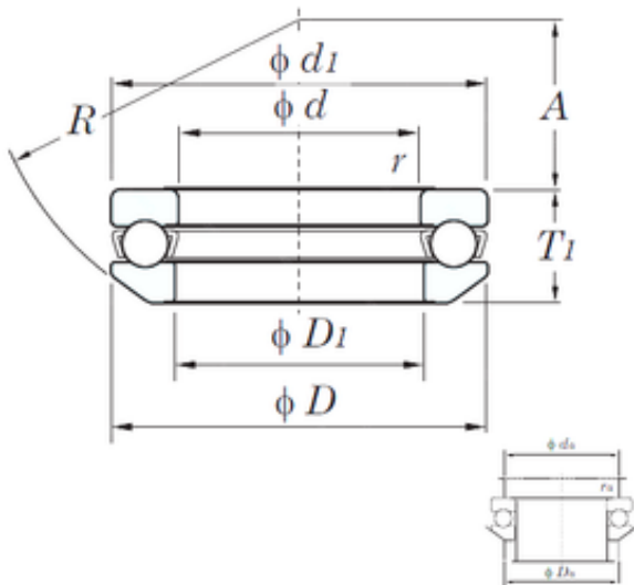
Bearing No. 53318
