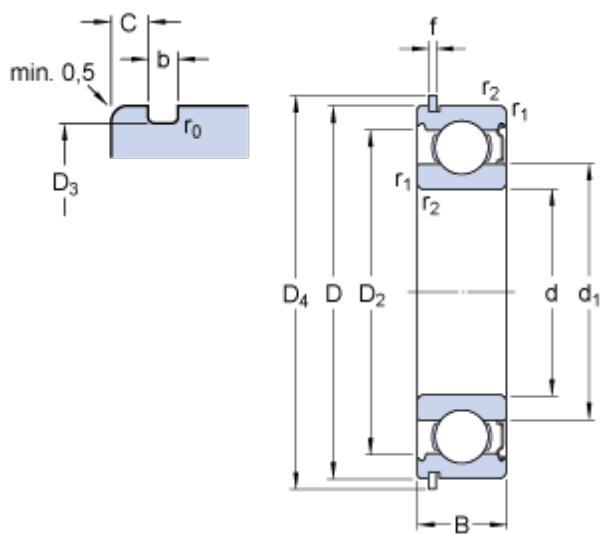
Bearing No. 6005-ZNR
