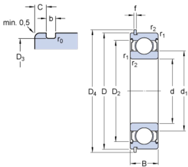
Bearing No. 6005-2ZNR
