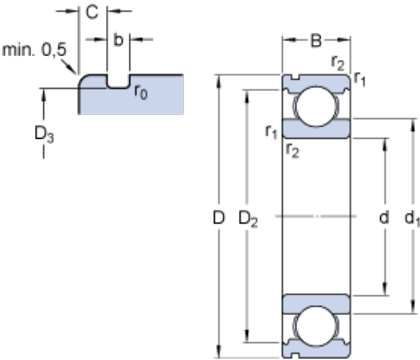
Bearing No. 6005 N
