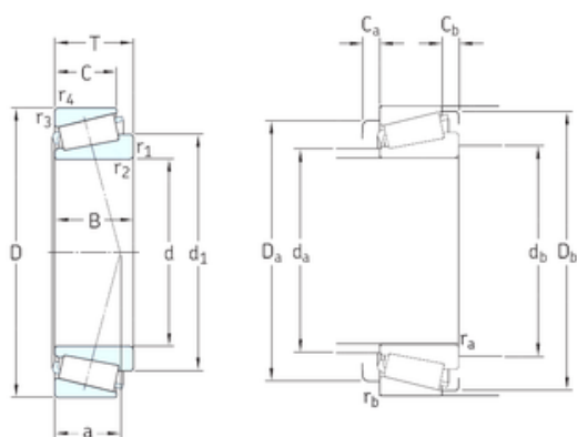
Bearing No. 30203J2
