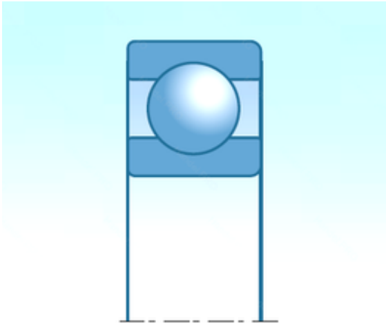
Bearing No. 6004HT200
