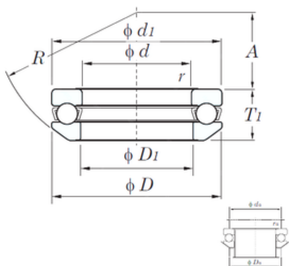
Bearing No. 53222
