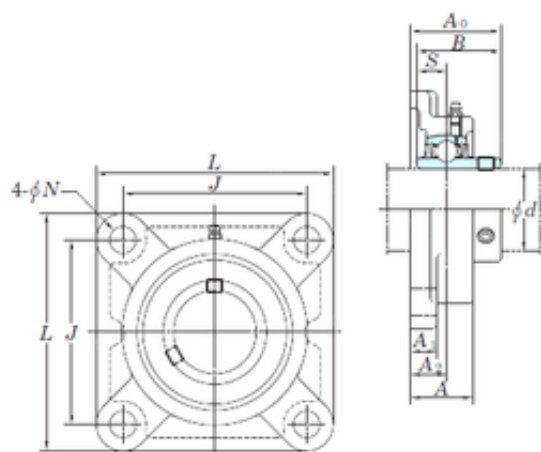
Bearing No. UCFX20
