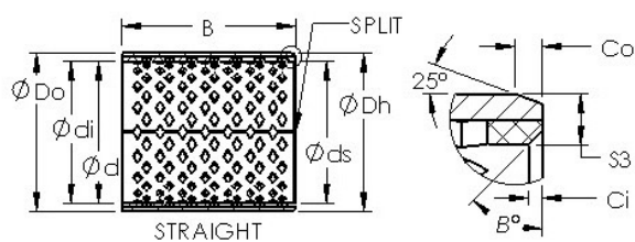
Bearing No. AST090 2220
