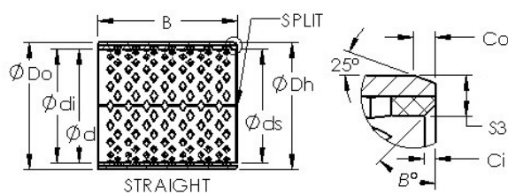
Bearing No. AST090 22070
