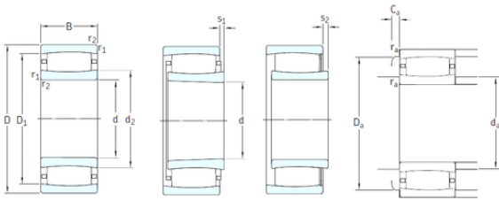
Bearing No. C30/900KMB
