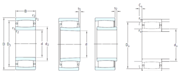
Bearing No. C2317K
