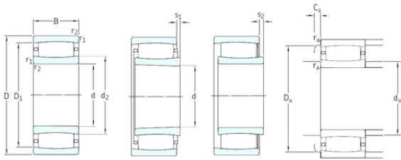
Bearing No. C2222K
