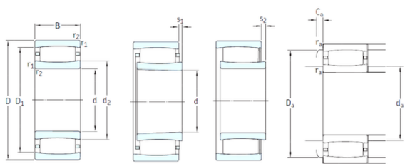
Bearing No. C2210KTN9
