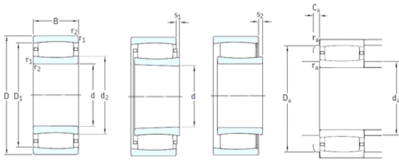
Bearing No. C2206TN9
