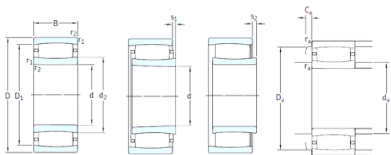
Bearing No. C2206KTN9
