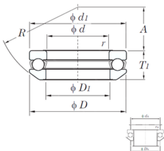
Bearing No. 53204
