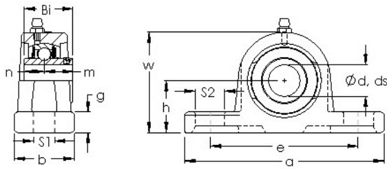
Bearing No. UCP 217
