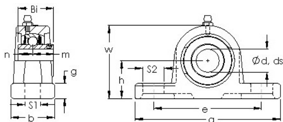
Bearing No. UCP 208
