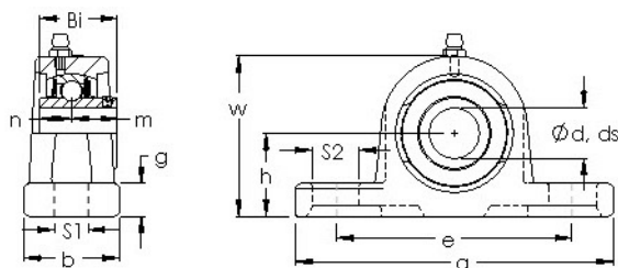
Bearing No. UCP 205
