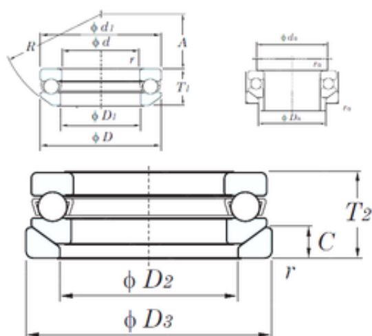
Bearing No. 53201U
