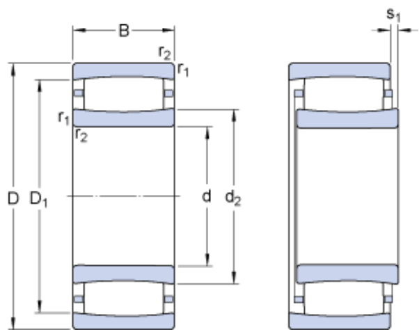
Bearing No. C 39/600 M
