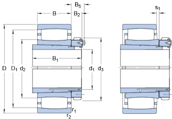
Bearing No. C 39/600 KM + OH 39/600 HE
