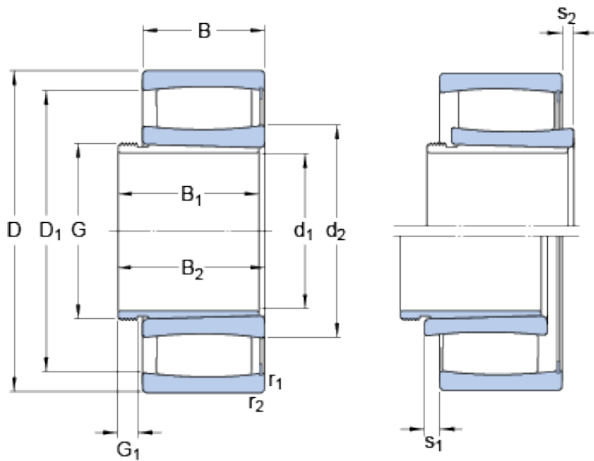
Bearing No. C 3138 KV + AH 3138 G
