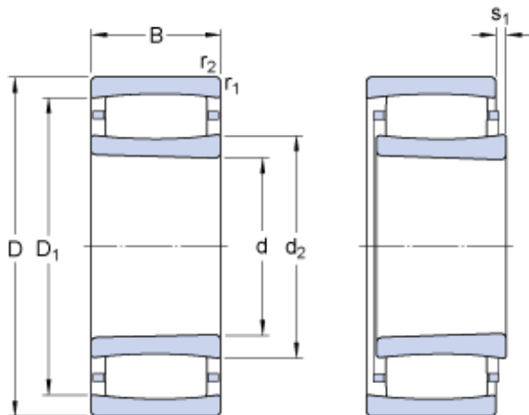
Bearing No. C 31/600 KMB
