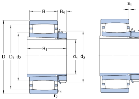
Bearing No. C 3038 K + H 3038
