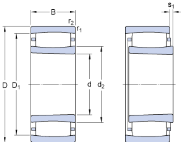
Bearing No. C 2213 KTN9
