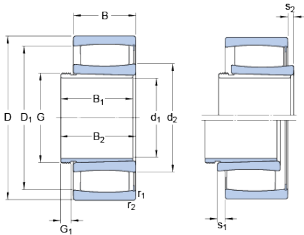
Bearing No. C 2209 KV + AH 309
