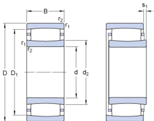
Bearing No. C 2207 TN9
